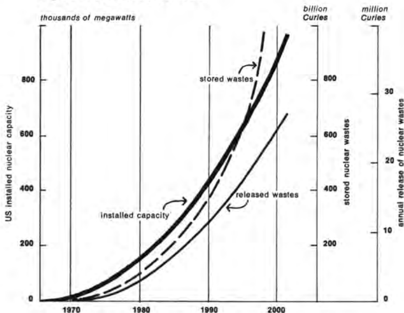
Figure 17 NUCLEAR WASTES
